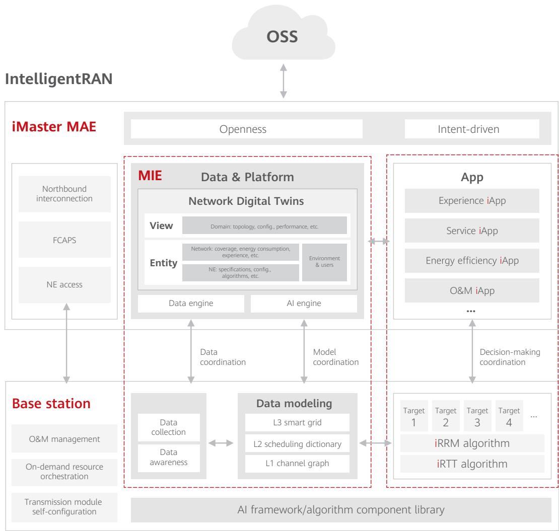
Figure 4-3 IntelligentRAN
