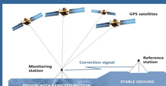
Fig. 9 RTK positioning technology
